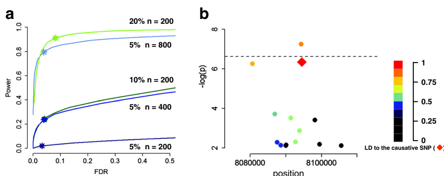
Figure 1 Sample size and effect size. a) Power and FDR for an idealized phenotype. Simulations in which a single random SNP explaining 5%, 10% or 20% of the phenotypic variance (with heritability \sim 0.75 ) were performed in either 200, 400 or 800 individuals [67]. Simulations are based on the available SNP data for Arabidopsis [20], with structure added by giving 10,000 random SNPs a tiny effects size. The star indicates power (the ability to find true positives) and FDR (false positives) at the 5% bonferroni-corrected threshold for 220,000 markers. b) An example of one particular simulation in which the causative SNP (red diamond) is not the most significant SNP in the local window. Remaining SNPs are colored according to their linkage to the causative SNP. Dashed line denotes the 5% bonferroni-corrected threshold for 220,000 markers.
